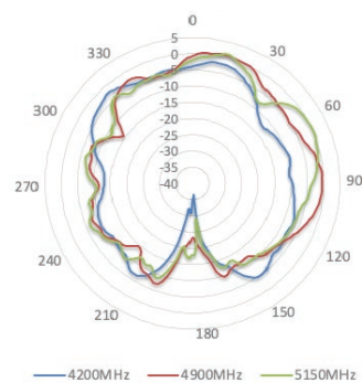
4200-5150 MHz
