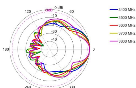
Elevation: 3400 – 3800 MHz
