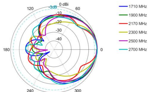
Elevation: 1710 – 2700 MHz
