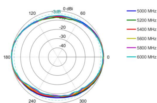
Elevation: 5000 – 6000 MHz
