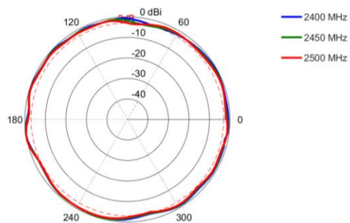
Elevation: 2400 – 2500 MHz
