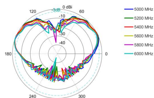
Elevation: 5000 – 6000 MHz
