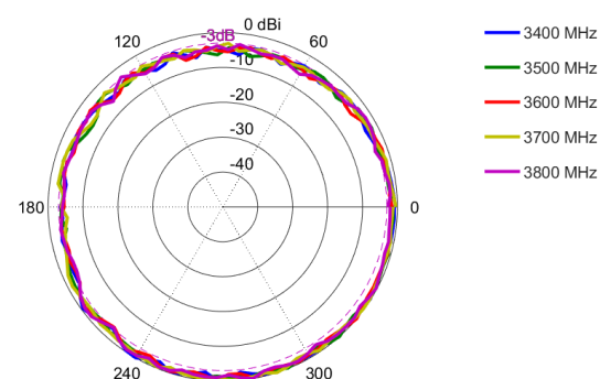
Azimuth (Top View): 3400–3800 MHz
